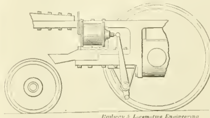
FIG. 1—BRAKE CYLINDER LOCATION.
